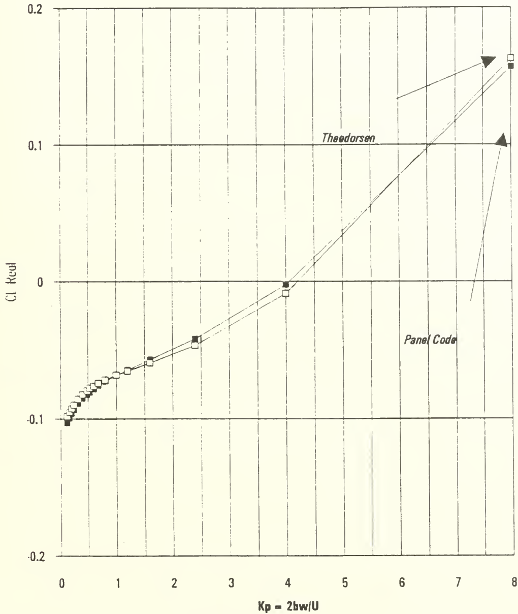
Real Part of C_I for Panel and Theodorsen (pitch, 1.0 deg, .37c, NACA0007, 75 panels top and bottom, 3cycles of 65 calc. per cycle)
